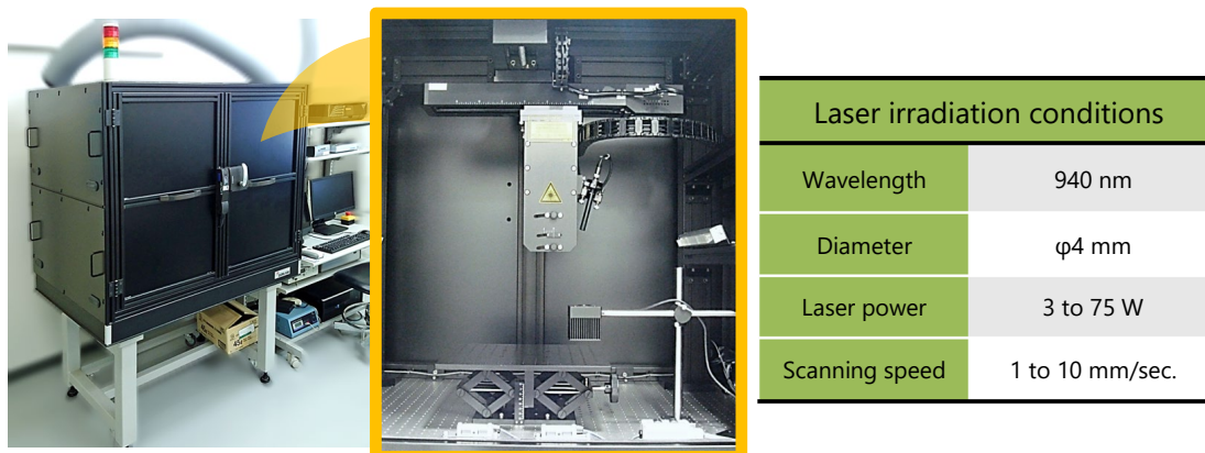
図 6 Example of experimental setup for laser adhesive system.
