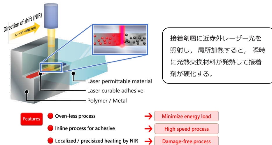
図 1 Laser Adhesive System.
