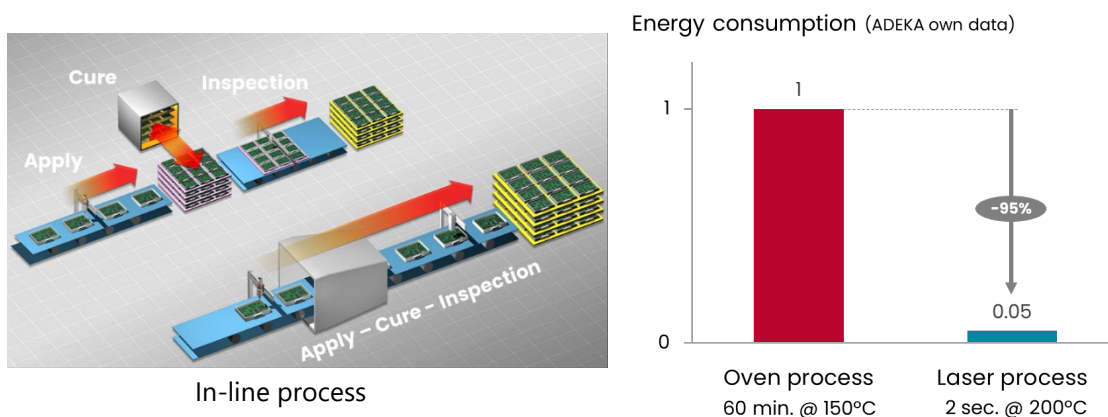
図 3 Benefits of laser and/or fast curing system
