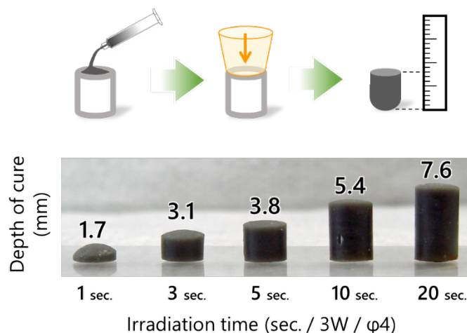
図 5 Results of deep curing test by laser irradiation.
