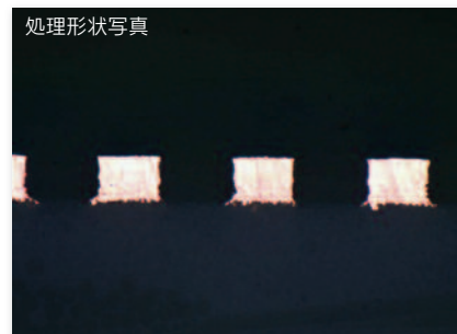
Circuit pitch 50 \mu m Cross Section
